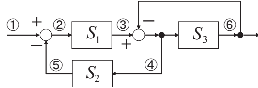
Fig. 1. Block Diagram of Control System
